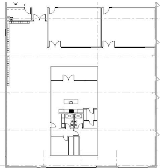
CONSTRUCTION SHOP FLOOR PLAN W/ EXAMPLE OF PRE-FAB HOME
